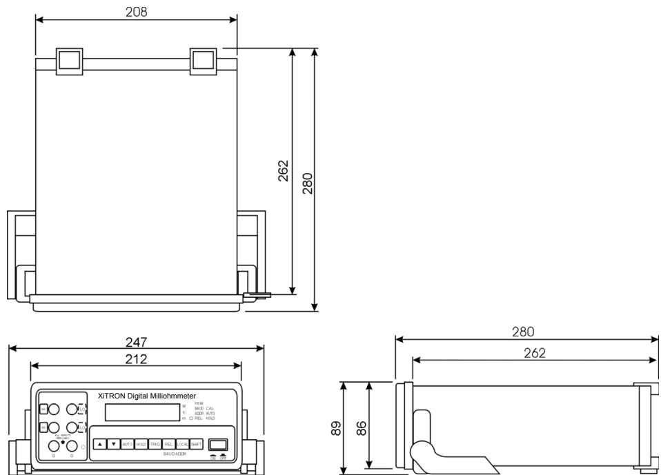
Figure 3. Meter Dimensions
