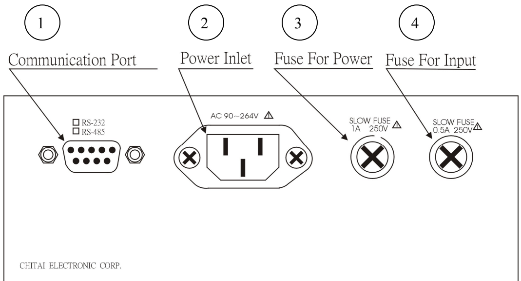
Figure 2. Rear Panel
