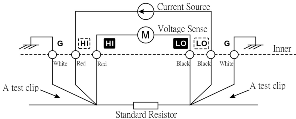
Figure 9. Calibration with Resistor Standard
